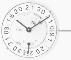
Small Second Cal. 6004.B 3.30 mm
